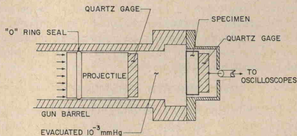
FIG. 2. Schematic diagram of the shock-wave experimental arrangement. In some of the experiments, the quartz gauge on the projectile is replaced by a facing of the specimen material.
